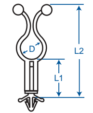
TO SNAP LOCK IN A .187 (4.8) DIA HOLE IN A 1/16" (1.6) NOMINAL THICK PANEL/BOARD (03-XX-SERIES)
